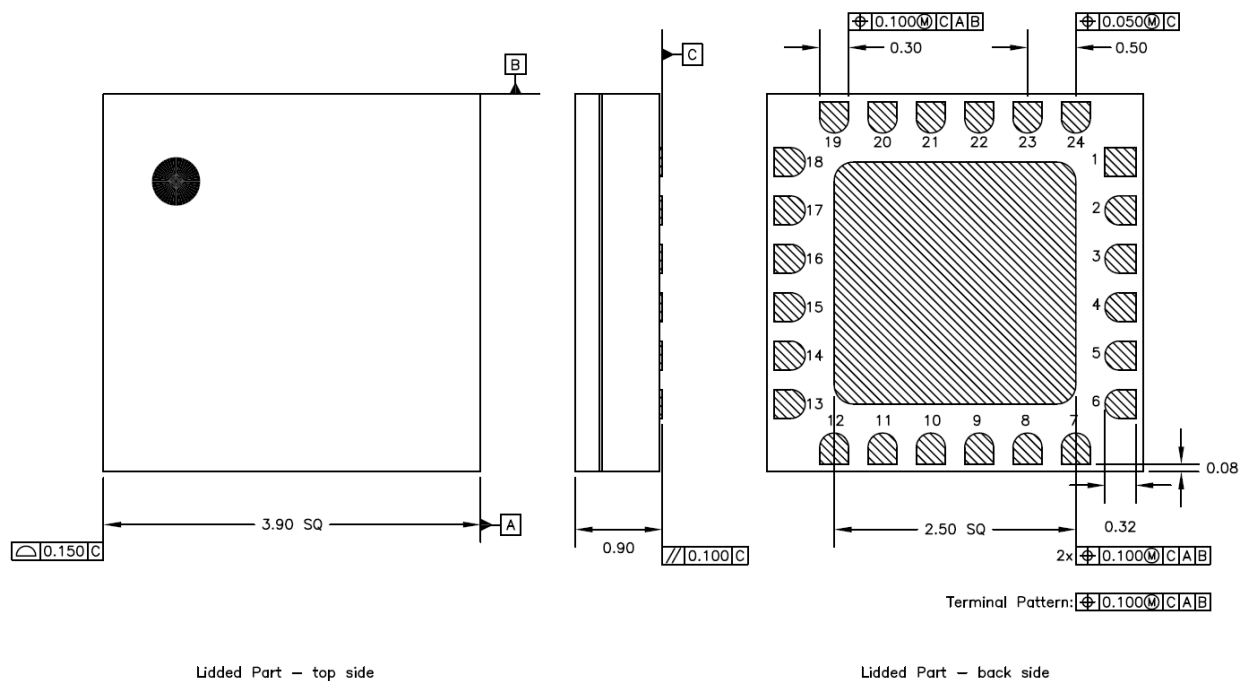
Figure 16 Package Outline
