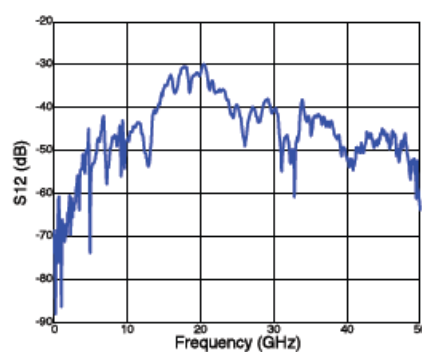
Figure 13 S-Parameters S12
