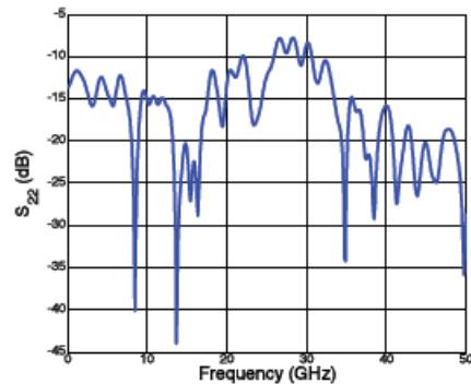
Figure 15 S-Parameters S22
