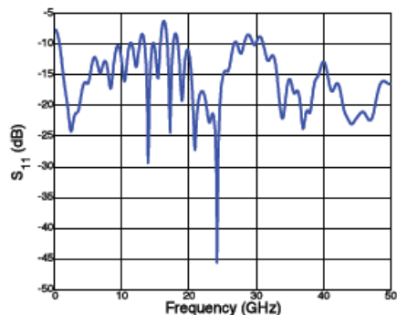
Figure 12 S-Parameters S11
