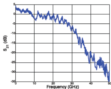
Figure 14 S-Parameters S21
