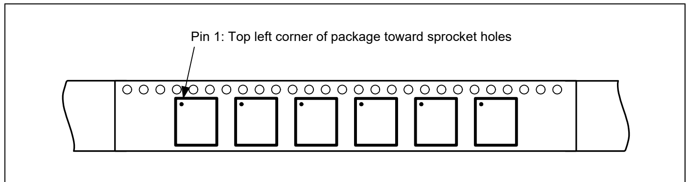
Figure 20. Pin 1 Orientation
