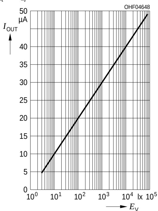
Output Current 2) page 13
