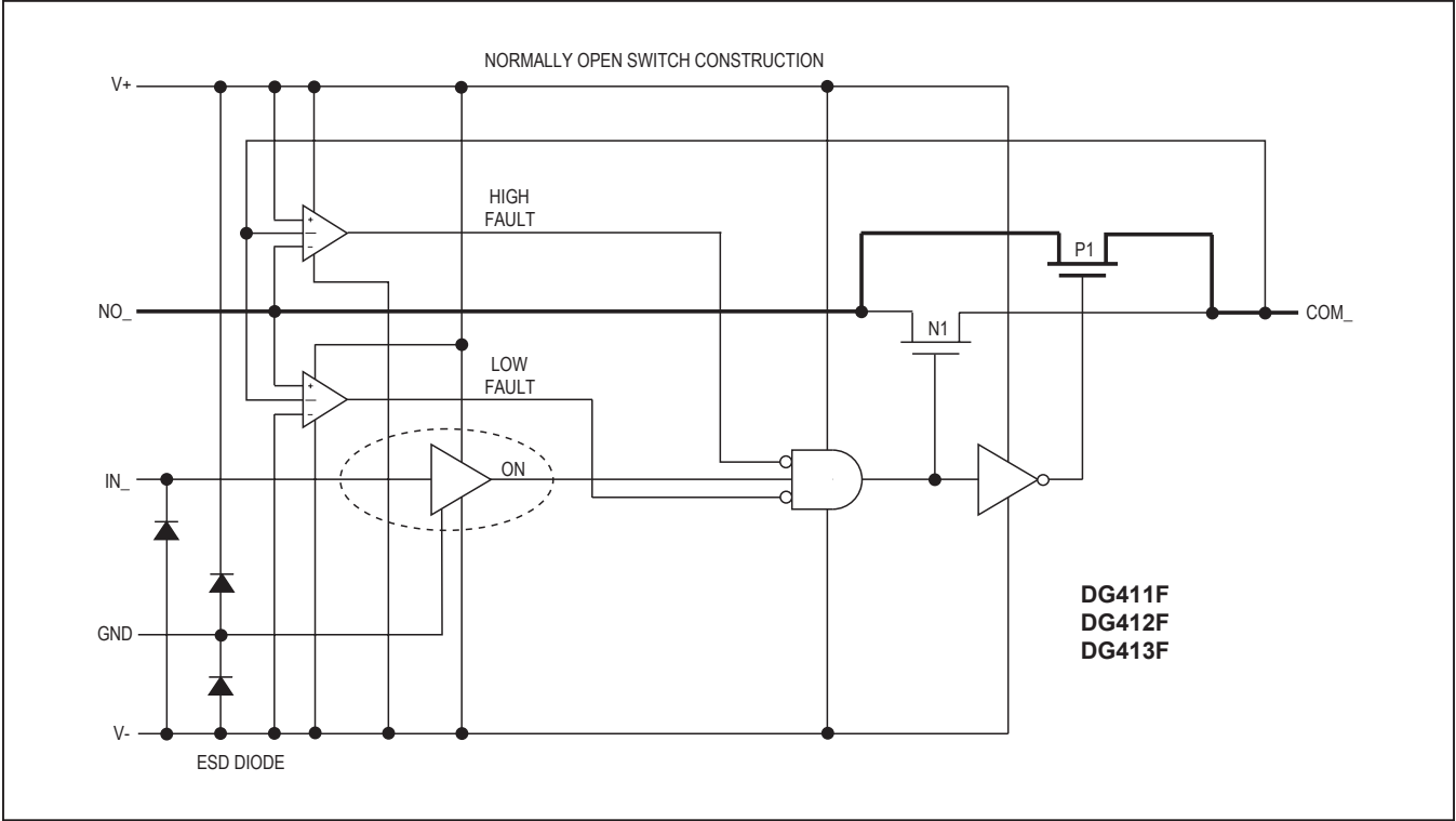
Figure 1. Functional Diagram
