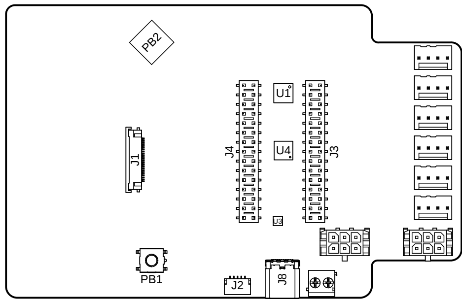
Arduino Braccio Carrier Top View
