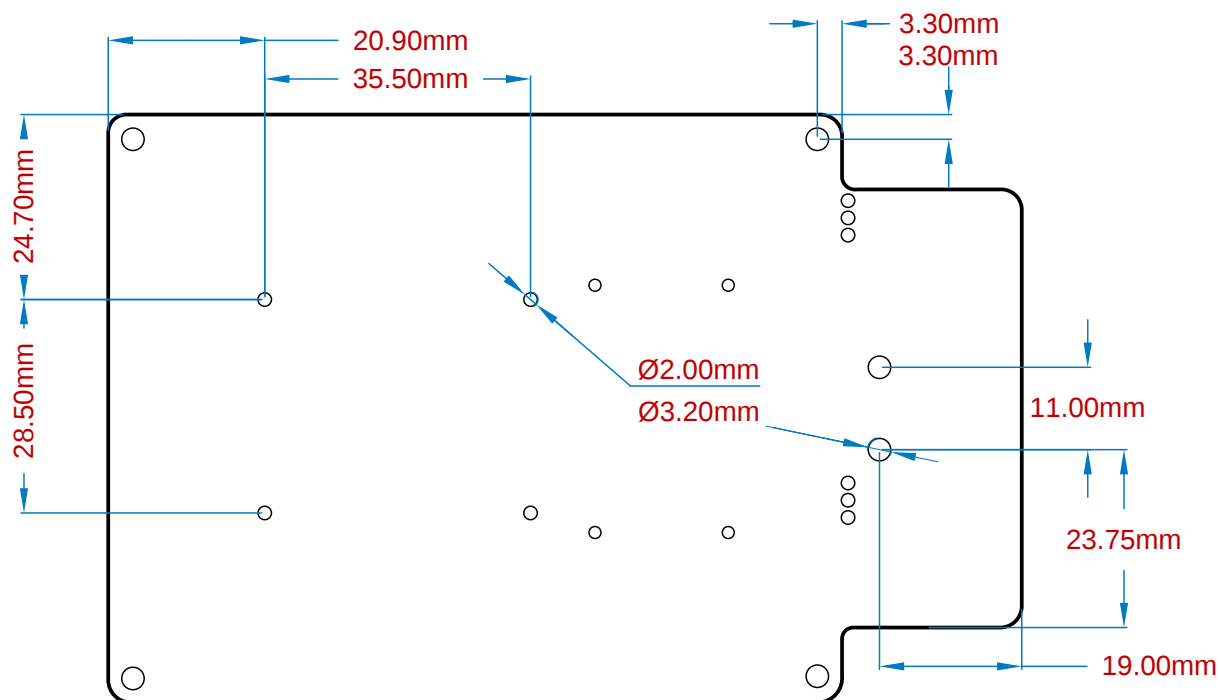
Mount Holes
