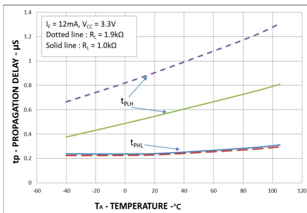
Figure 6: Typical Propagation Delay vs. Temperature, 3.3V
