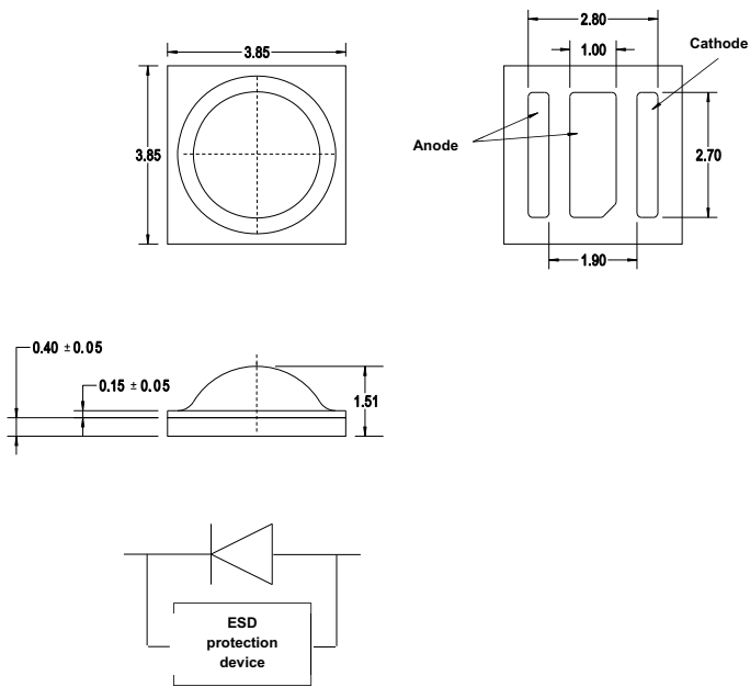
Figure 1: Package Drawing
