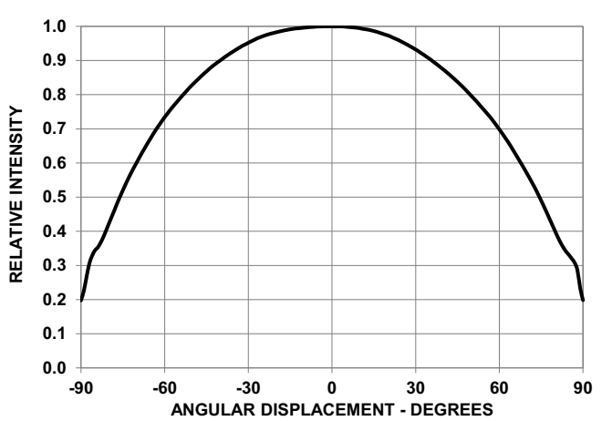
Figure 7: Radiation Pattern
