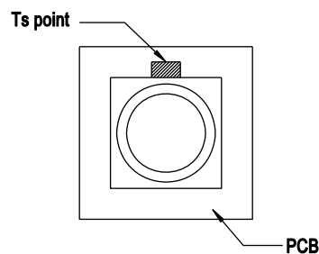
Figure 14: Solder Point Temperature on PCB
