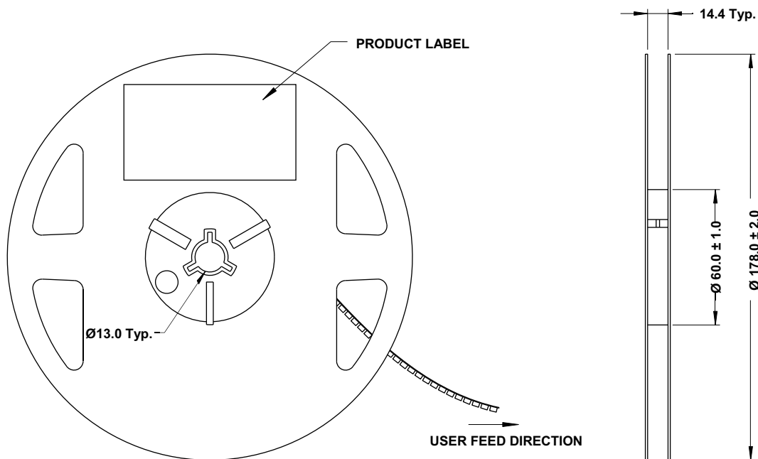
Figure 12: Reel Dimensions
