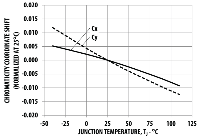
Figure 14: Chromaticity Coordinate Shift vs. Junction Temperature for 6500K
