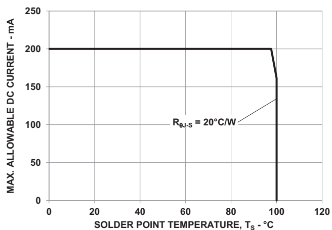
Figure 16: Maximum Forward Current vs. Solder Point Temperature. Derated based on T_{JMAX} = 110^{\circ}\text{C} , R_{\theta J-S} = 20^{\circ}\text{C/W} .
