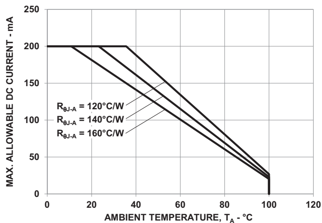
Figure 15: Maximum Forward Current vs. Ambient Temperature. Derated based on T_{JMAX} = 110^{\circ}\text{C} , R_{\theta J-A} = 120^{\circ}\text{C/W} , 140^{\circ}\text{C/W} and 160^{\circ}\text{C/W} .
