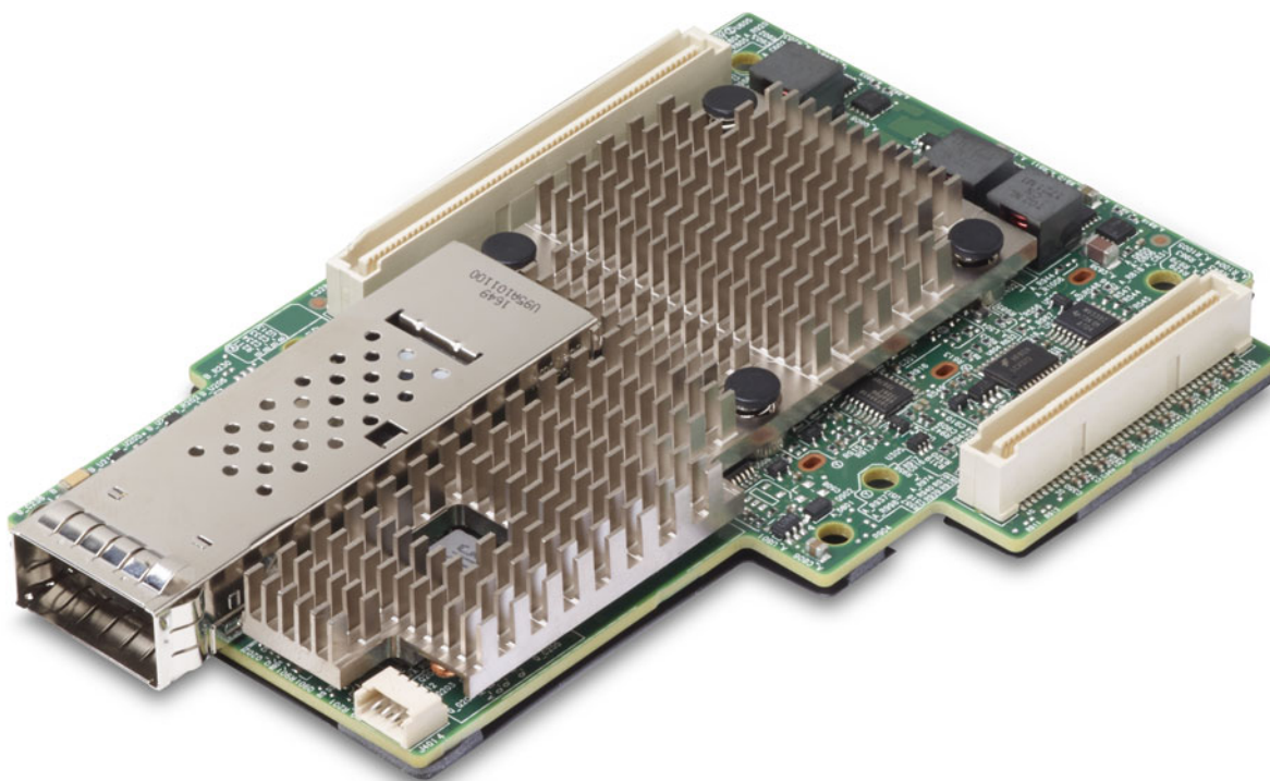
Figure 1: BCM957454M4540C OCP Mezzanine Card
