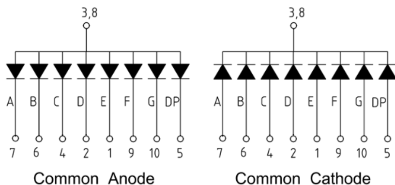
Figure 2: Circuit Diagram
