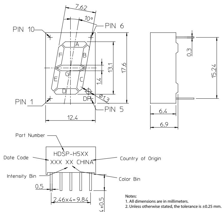
Figure 1: Package Dimensions
