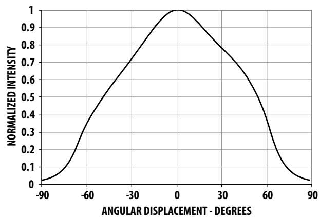
Figure 6 Radiation Pattern, Major Axis
