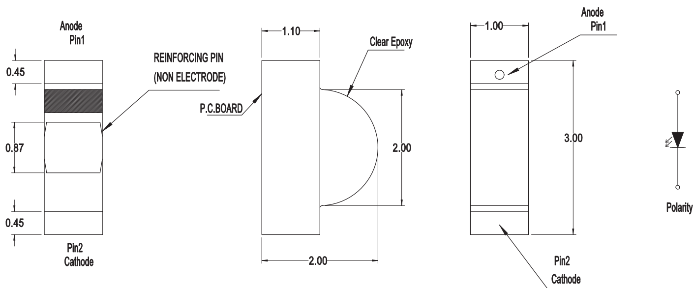
Figure 1: Package Dimensions
