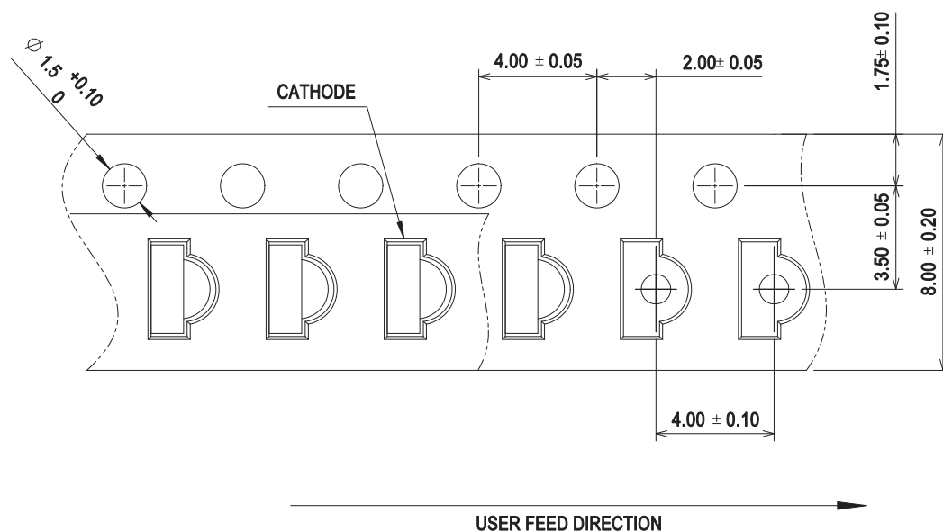
Figure 8: Carrier Tape Dimensions
