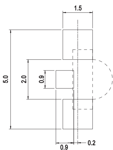
Figure 7: Recommended Soldering Land Pattern
