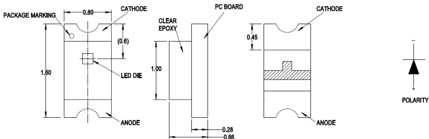
Figure 1: Package Dimensions
