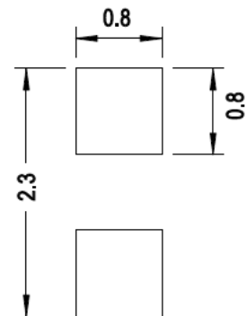
Figure 7: Recommended Soldering Land Pattern
