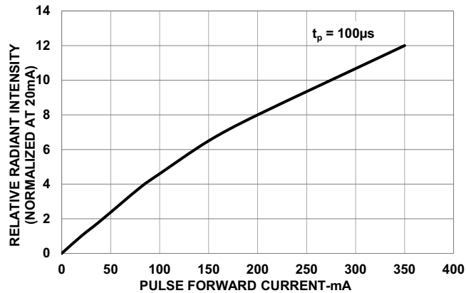
Figure 4: Relative Radiant Intensity vs. Forward Current
