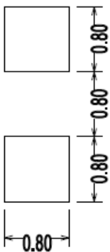
Figure 7: Recommended Soldering Land Pattern
