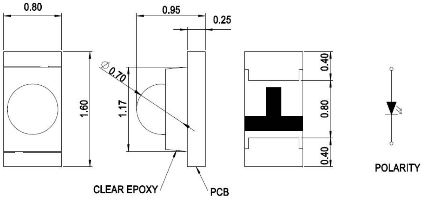
Figure 1: Package Dimensions
