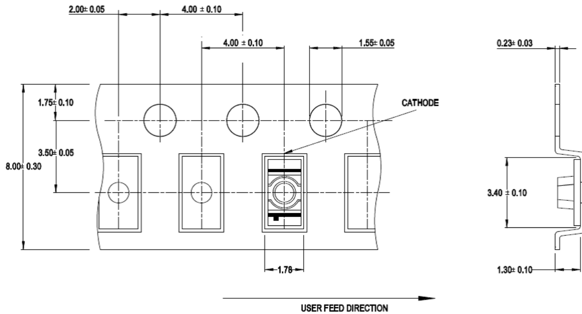
Figure 7: Carrier Tape Dimensions
