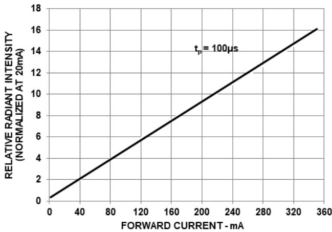
Figure 3: Relative Radiant Intensity versus Forward Current
