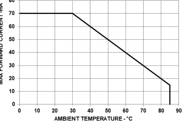
Figure 5: Derating Curve
