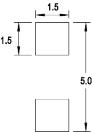
Figure 6: Recommended Soldering Land Pattern
