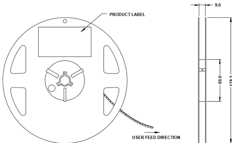
Figure 8: Reel Dimensions
