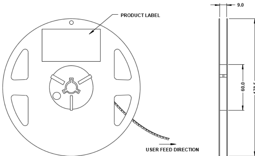
Figure 8: Reel Dimensions
