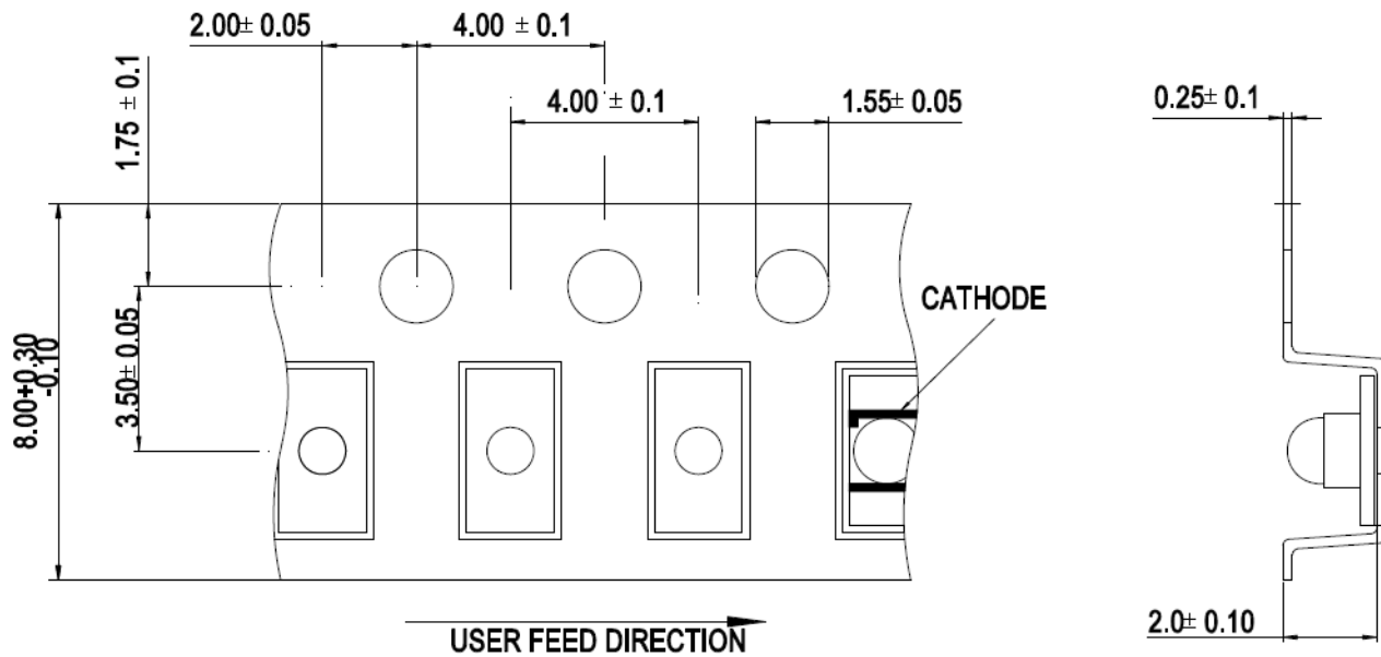
Figure 7: Carrier Tape Dimensions
