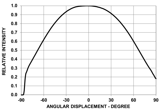
Figure 5: Radiation Pattern
