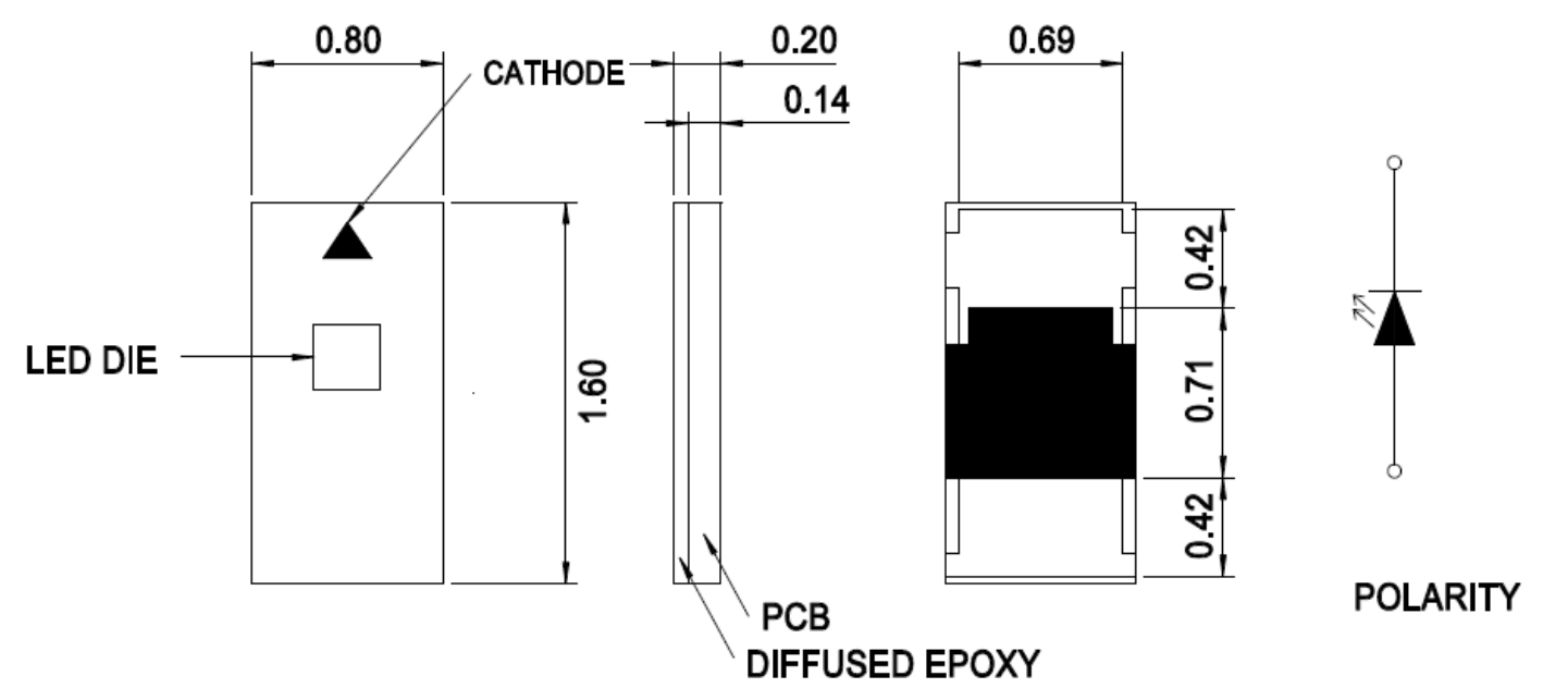
Figure 1: Package Dimensions
