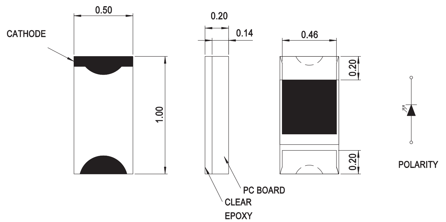
Figure 1: Package Dimensions
