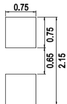
Figure 7: Recommended Soldering Land Pattern
