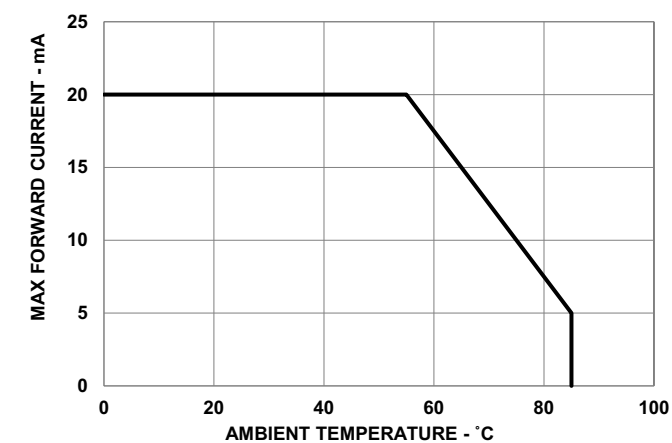
Figure 6: Derating Curve
