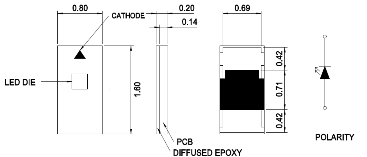
Figure 1: Package Dimensions
