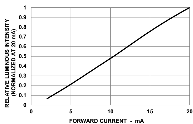
Figure 4: Relative Luminous Intensity vs. Forward Current
