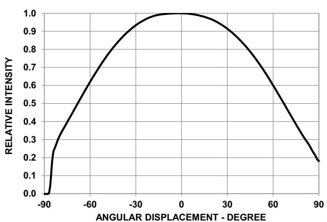
Figure 5: Radiation Pattern
