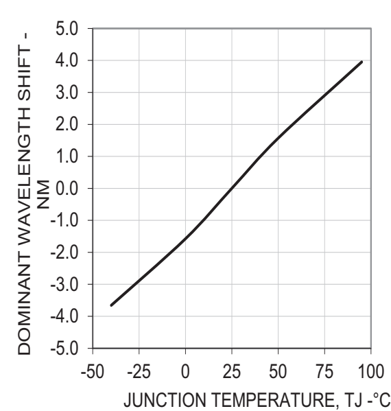
Figure 9: Wavelength Shift vs. Temperature
