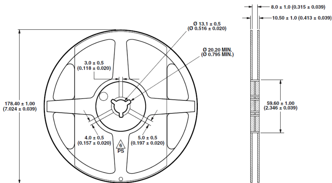
Figure 13: Reel Dimensions
