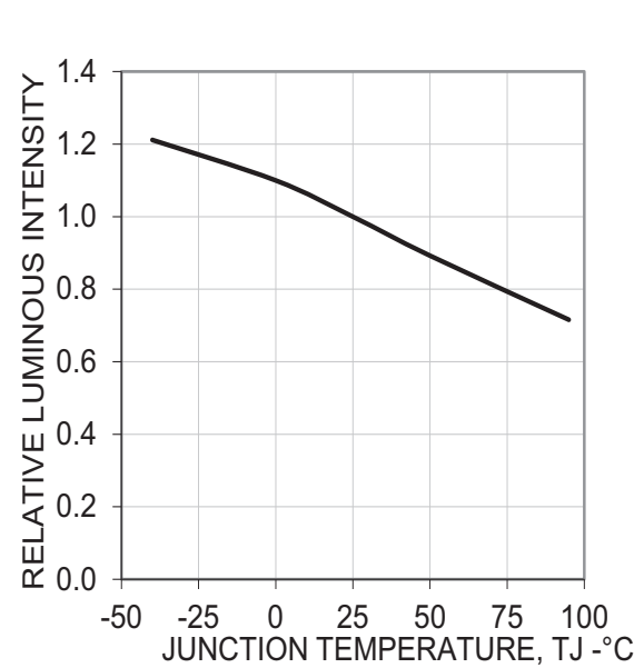
Figure 7: Relative Intensity vs. Temperature
