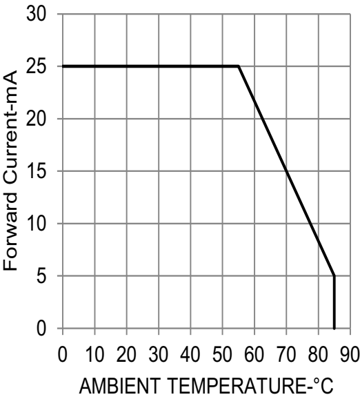
Figure 10: Derating Curve
