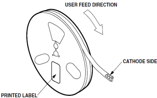
Figure 12: Reel Orientation
