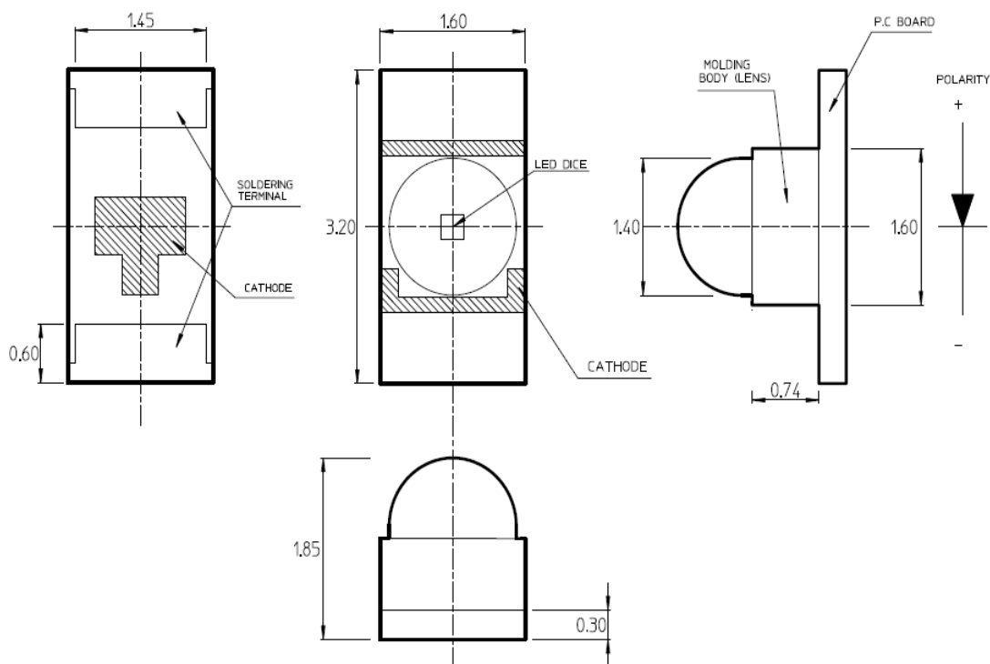
Figure 1: Package Dimensions
