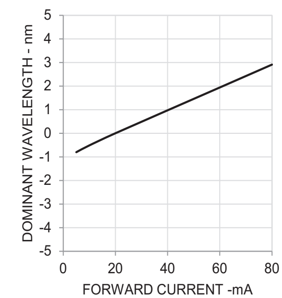
Figure 6: Wavelength Shift vs. Forward Current
