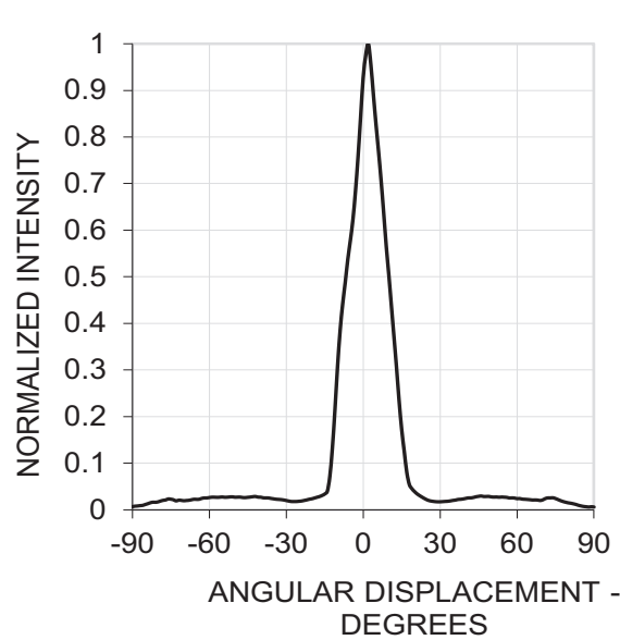
Figure 5: Radiation Pattern
