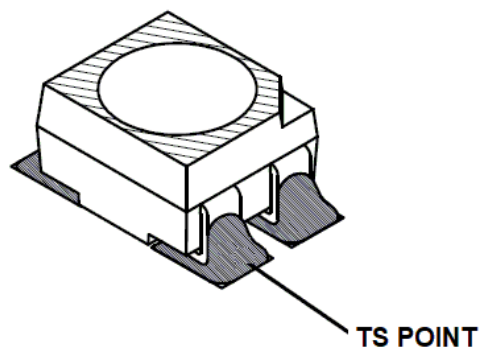
Figure 14: Solder Point Temperature on PCB
