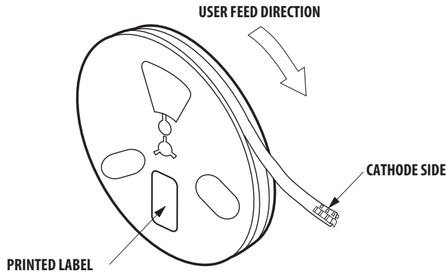
Figure 11: Reeling Orientation
