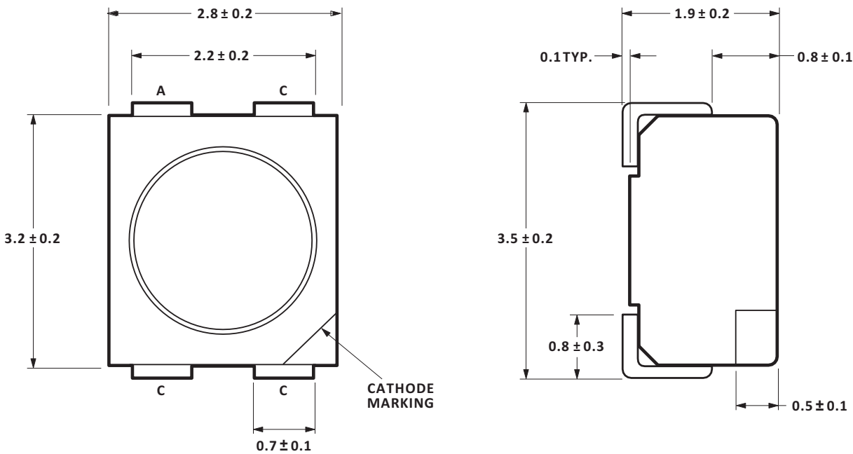
Figure 1: Package Dimensions
