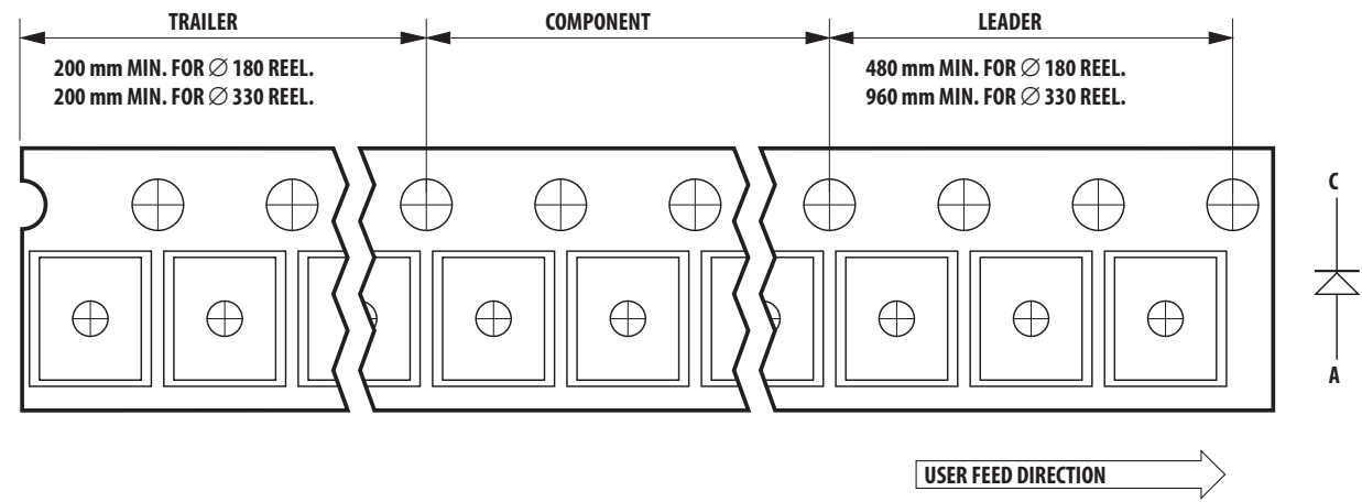
Figure 9: Tape Leader And Trailer Dimensions
