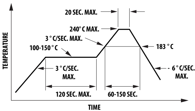
Figure 6: Recommended SnPb Reflow Soldering Profile
