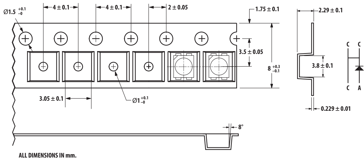
Figure 11: Reeling Orientation
