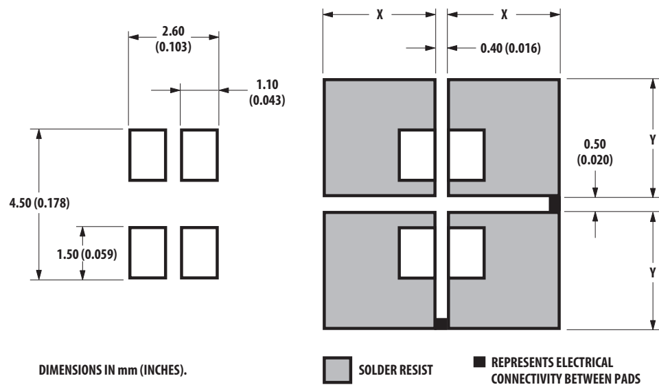
Figure 8: Recommended Soldering Pad Pattern
