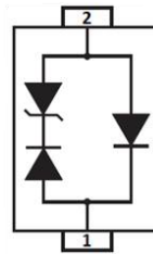
Device Schematic
