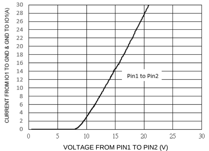
Figure 8. TLP Curve (tp = 100ns)
