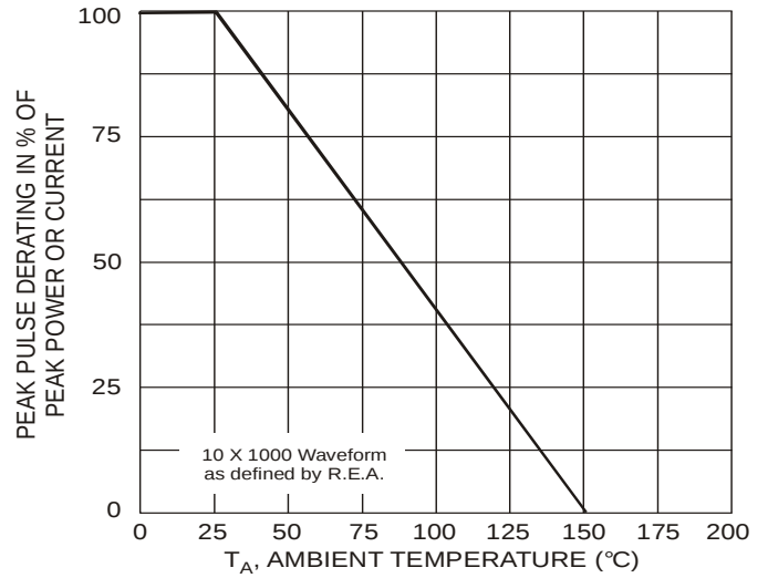
Figure 4. Peak Pulse Power vs. T_A
