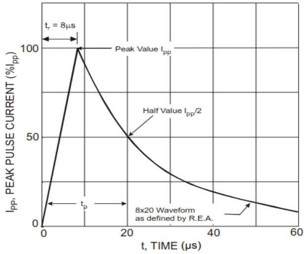
Figure 3. Typical 8 x 20μs Pulse Waveform
