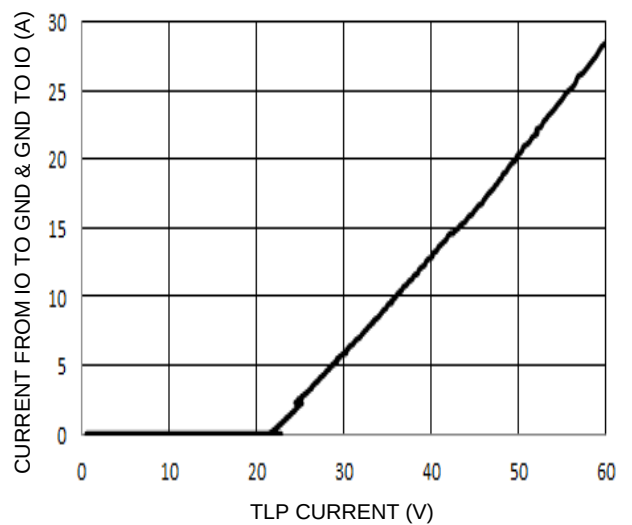
Figure 8. TLP Curve ( t_P = 100ns )
