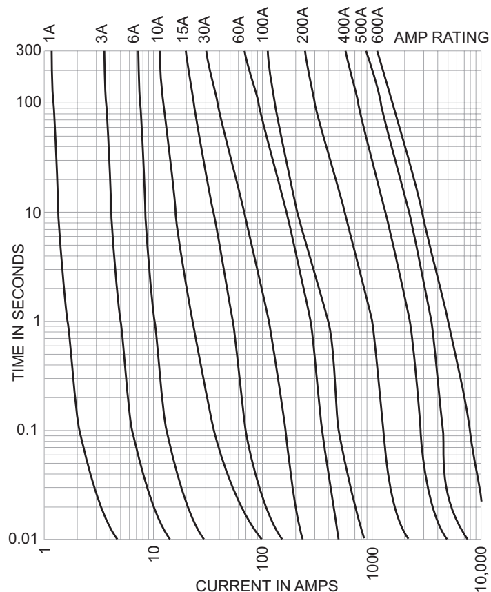
JJS Time-current characteristics — average melt
