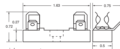
2499 side 1/4" quick-connect
