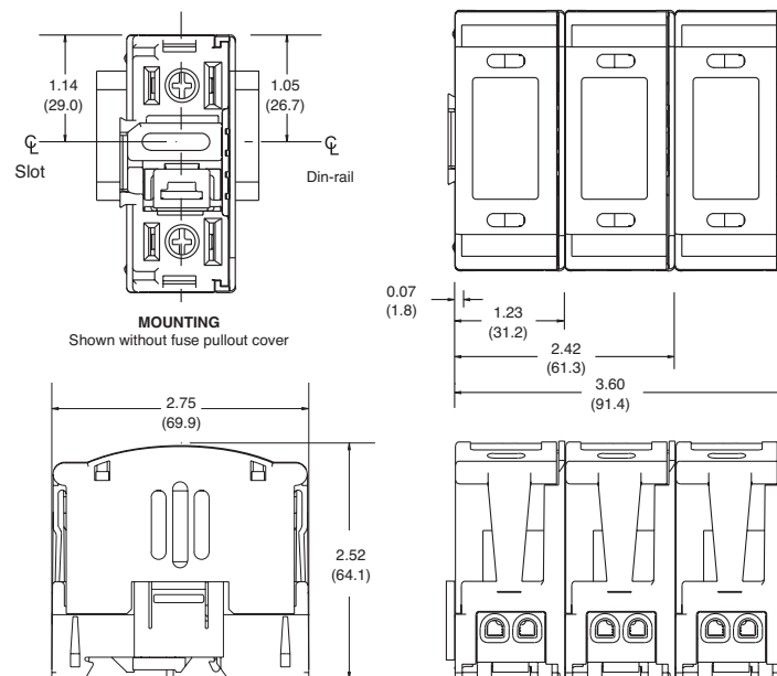
JT(N)60030
