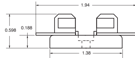
4520 integral clip and straight solder terminals
