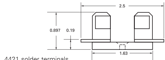
4421 solder terminals
