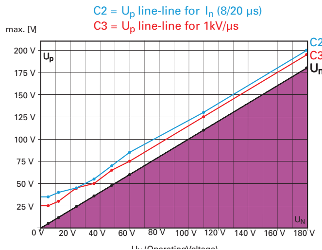
Diagram 1: voltage protection level U_p (V) (line-line)
