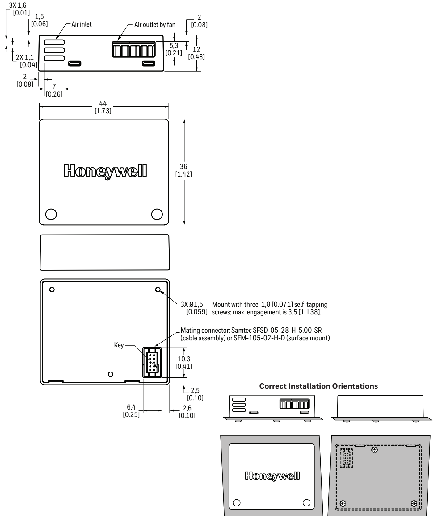
Figure 3. Compact Version HPM115CO-003 Mounting Dimensions and Correct Installation Orientations (For reference only: mm/[in])
