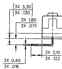
LEFT ANGLE TERMINALS
