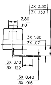
RIGHT ANGLE TERMINALS
