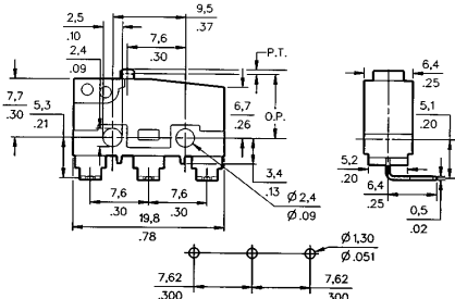
Lever Actuators 4mm (.158) wide
