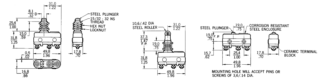
Fig. 1 Mounting holes will accept pins or screws of .139" (3,53 mm) dia.
