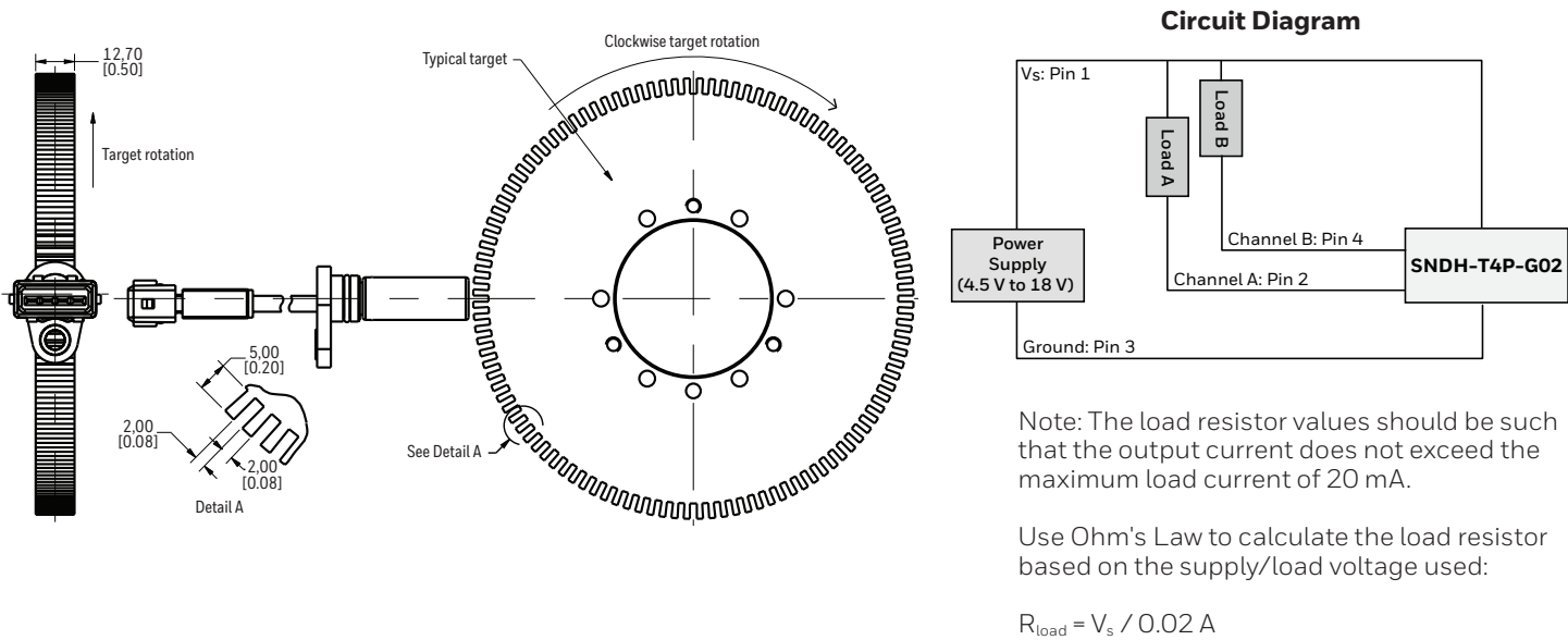
Figure 6. SNDH-T4P-G02 Dimensional Drawings (For reference only: mm [in])
