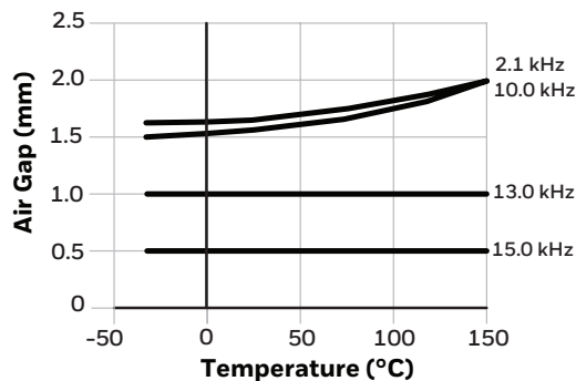
Figure 2. Temperature Air Gap Frequency Derating Curve
