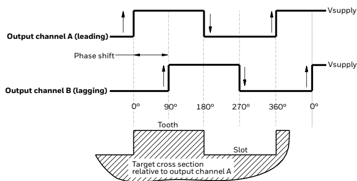
Figure 1. Sensor Output
