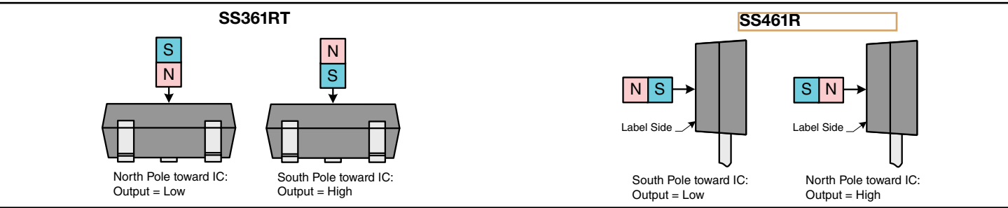
Figure 4. Magnetic Activation
