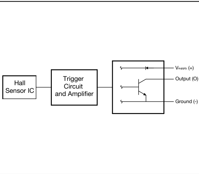
Figure 4. Magnetic Activation
