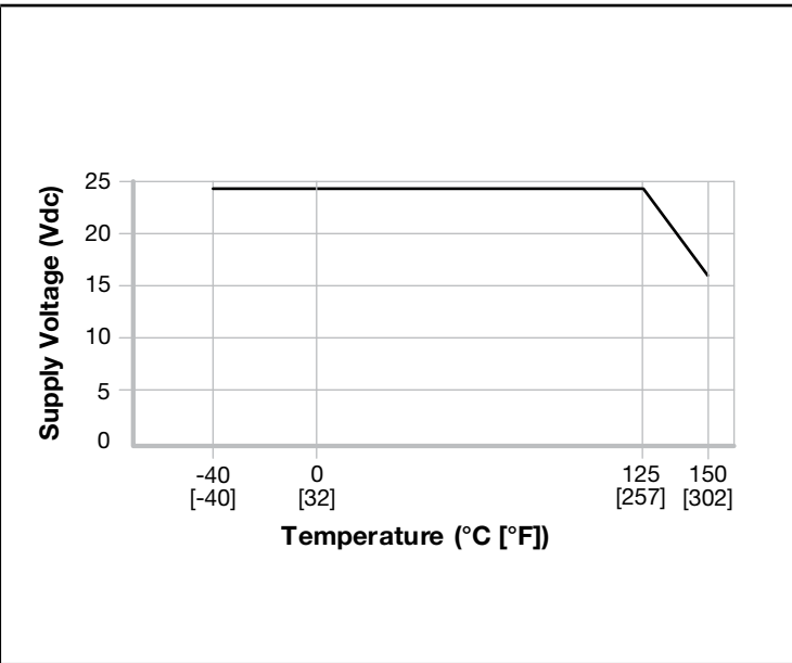
Figure 3. SS361RT Rated Supply Voltage
