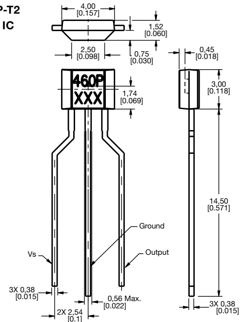
Figure 6. SS460P Sensor IC, SS460P-T2 Sensor IC and Ammopack Tape-in-Box Mounting Dimensions (For reference only. mm/in.)
