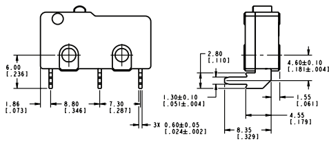
Terminal Type 60 - Left PCB
