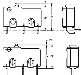
Operate Point References for PCB Terminals
