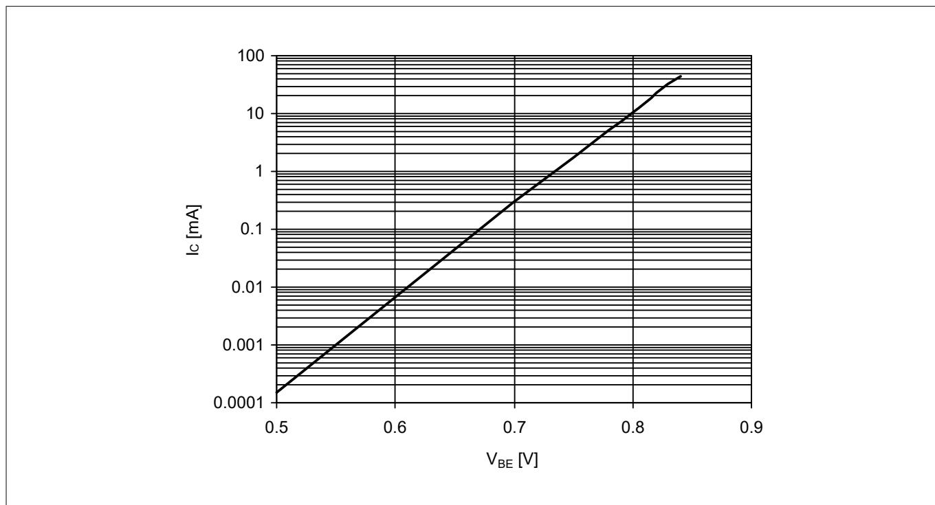
Figure 5 Collector current vs. base emitter voltage I_C = f(V_{BE}) , V_{CE} = 2 V
