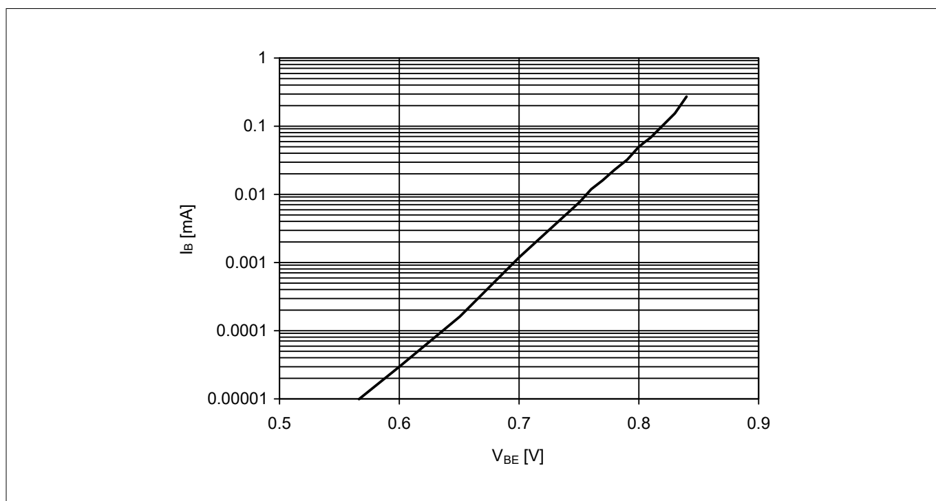
Figure 6 Base current vs. base emitter forward voltage I_B = f(V_{BE}) , V_{CE} = 2 V
