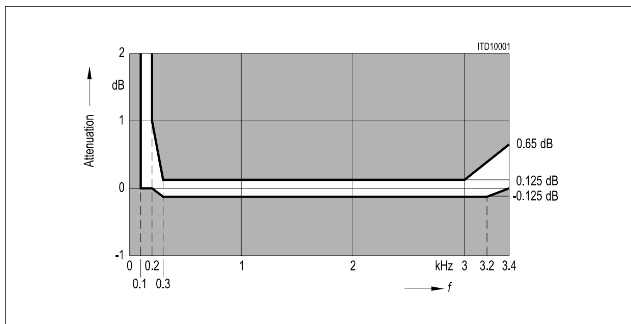
Figure 16 Transmit
