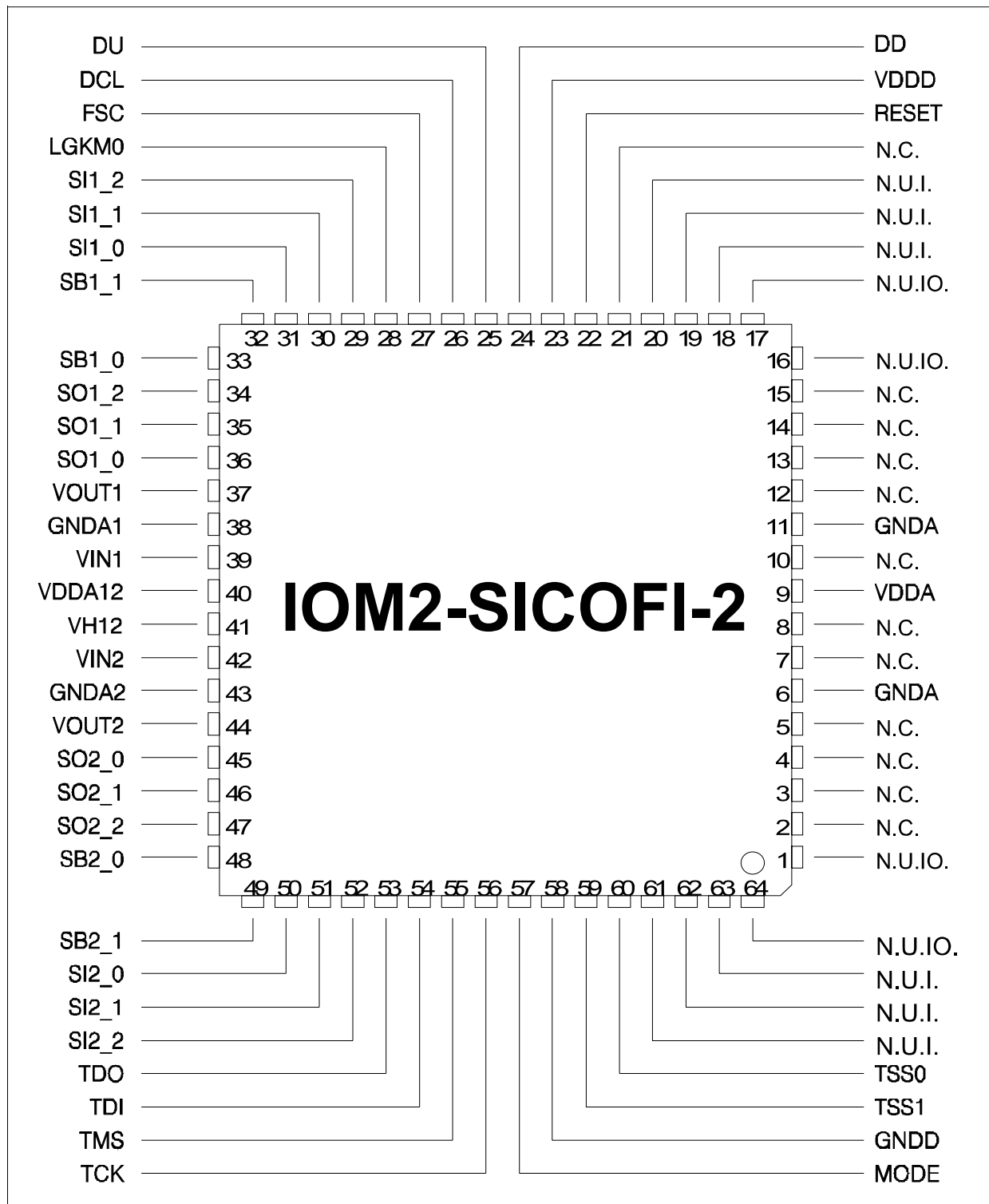
Figure 1 Pin Configuration
