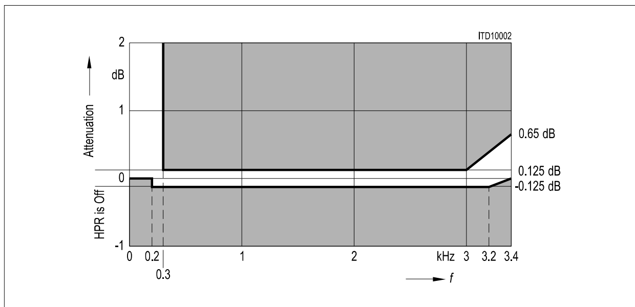
Figure 15 Receive
