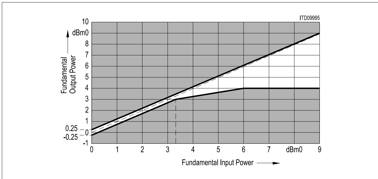
Figure 22 Overload Compression
