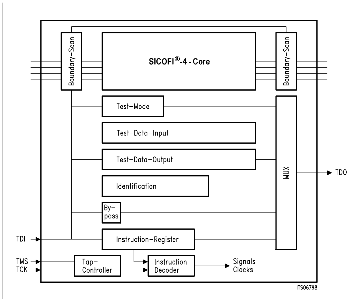
Figure 35 TAP-Controller
