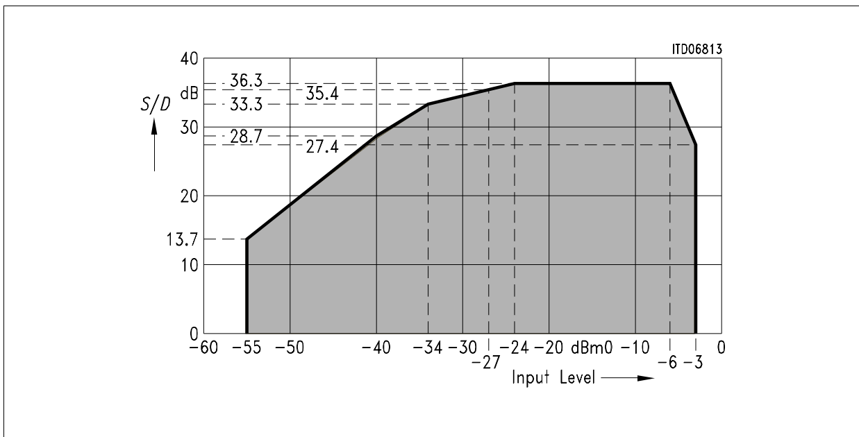
Figure 26 Transmit
