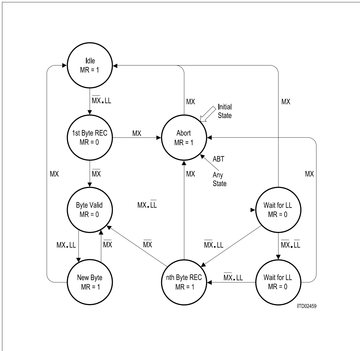
Figure 34 State Diagram of the IOM-2 SICOFI-2 Monitor Receiver
