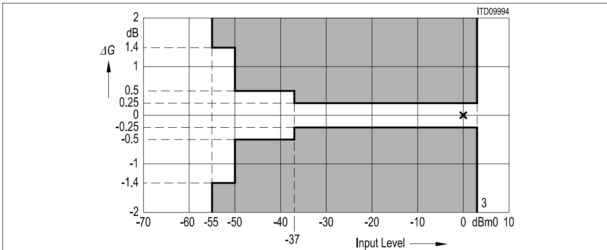
Figure 23 Gain Tracking
