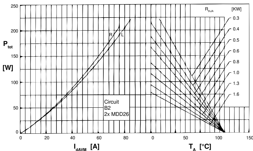
Fig. 6 Single phase rectifier bridge: Power dissipation vs. direct output current I_dAVM and ambient temperature; R = resistive load, L = inductive load
