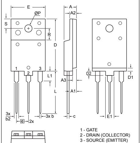
X017c TO-3PFP Weight = 5.5 g
