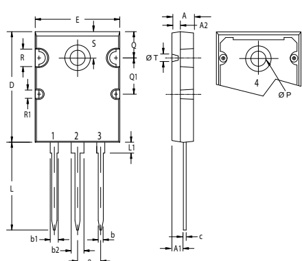
X020a TO-264 AA Weight = 10 g
