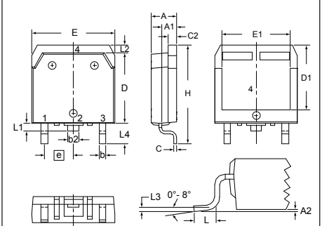
X019 TO-268 AA (D 3 PAK) Weight = 4 g
