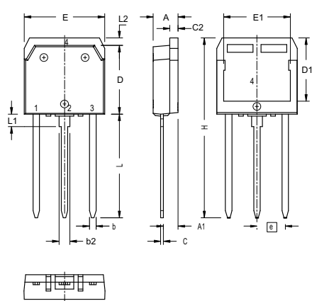
X018 TO-268 I 3 PAK Weight = 4.5 g
