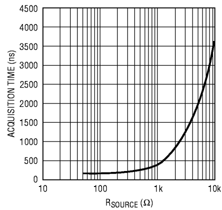
Acquisition Time vs Source Impedance
