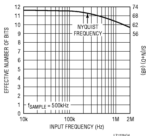
Effective Bits and Signal-to-(Noise + Distortion) vs Input Frequency
