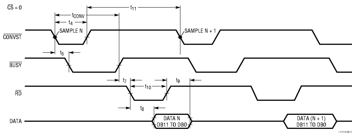
Figure 14. Mode 2. \overline{CONVST} Starts a Conversion. Data is Read by \overline{RD}
