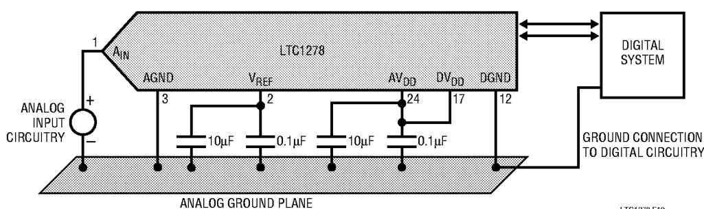
Figure 10. Power Supply Grounding Practice
