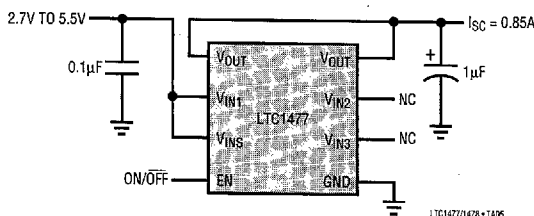
0.85A Protected Switch
