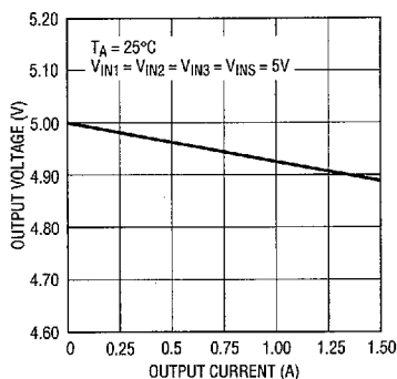
Switch Output Voltage
