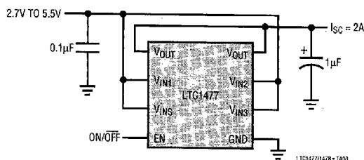
2A Protected Switch
