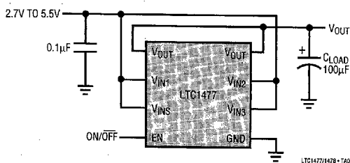
2A Protected Switch Driving a Large Capacitive Load
