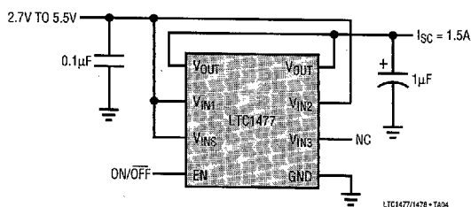
1.5A Protected Switch
