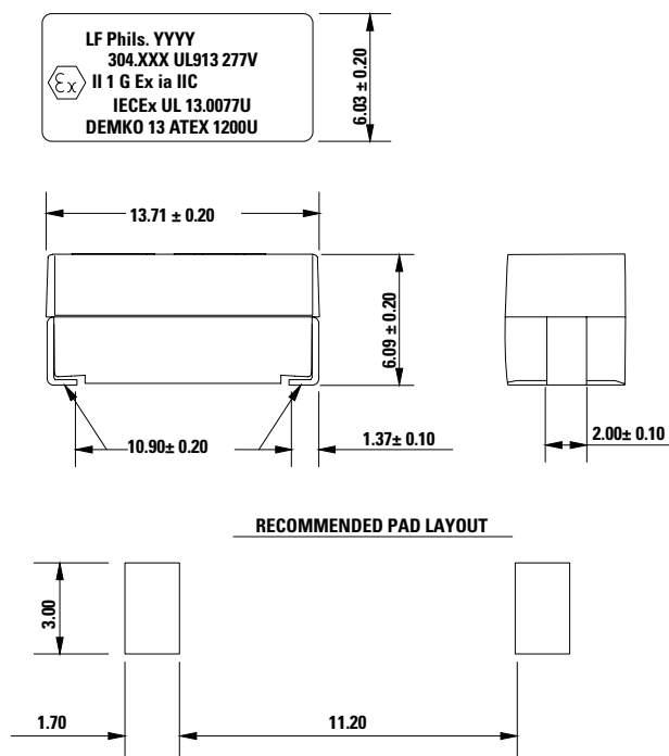
Dimensions (mm)
