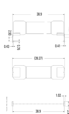
ZXPCBL PCB Mount (Long)
