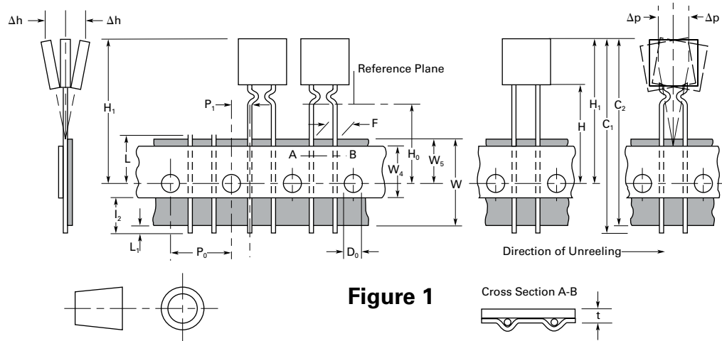
Tape and Reel Diagrams
