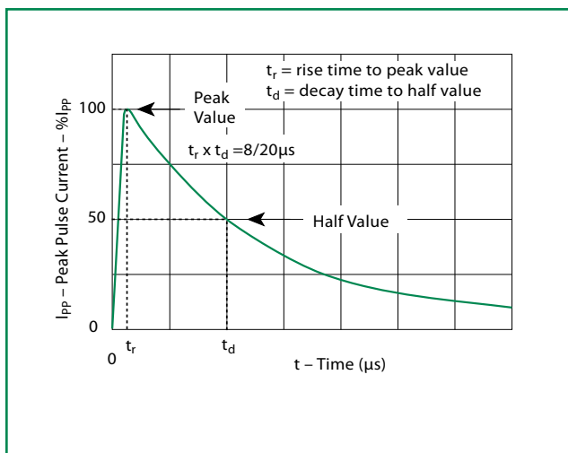
Figure 8 - Pulse Waveform
