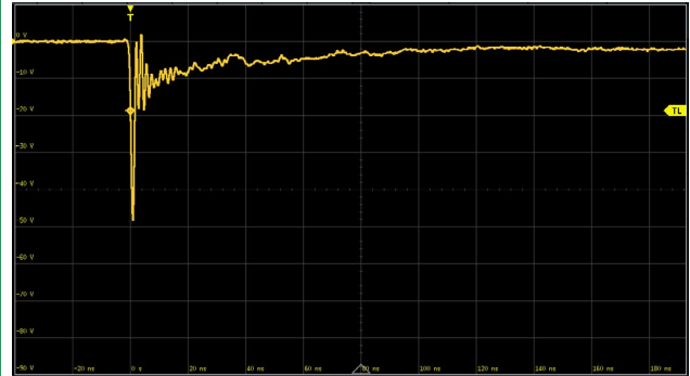
IEC 61000-4-2 -8 kV Contact ESD Clamping Voltage
