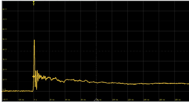
IEC 61000-4-2 +8 kV Contact ESD Clamping Voltage
