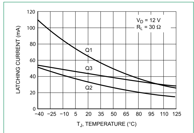
Figure 10. Latching Current Variation
