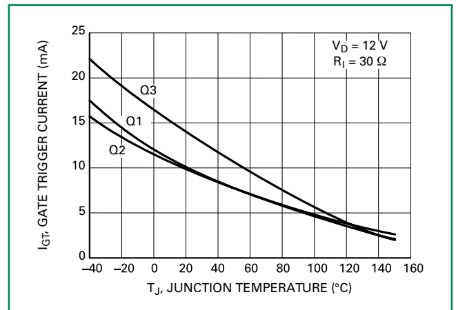
Figure 5. Gate Trigger Current Variation
