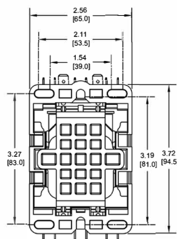
3 Pole Contactor 50 - 60 FLA
