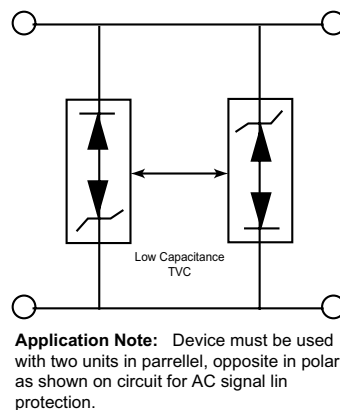
Figure 4 - AC Line Protection Application
