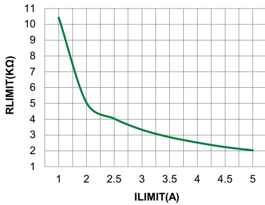
Figure 1. Programmable Current Limit ( V_{IN}=3.3V, 5V and 12V )
