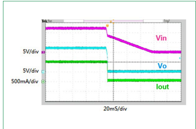
Figure 7. Shutdown (12V Mode, I_O=1A , C_{SS}=100nF )
