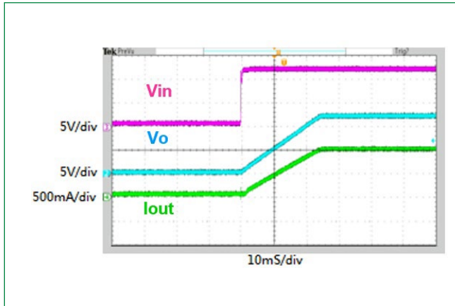
Figure 7. Programmable Soft-start Time (12V Mode, I_O=1A , C_{SS}=100nF )
