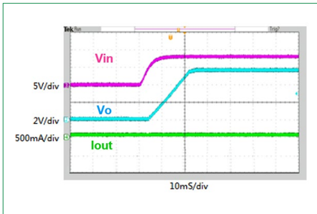
Figure 8. Over Voltage Protection (5V Mode, V_{IN}=8V , I_O=0A )
