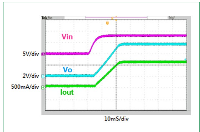
Figure 9. Over Voltage Protection (5V Mode, V_{IN}=8V , I_O=1A )
