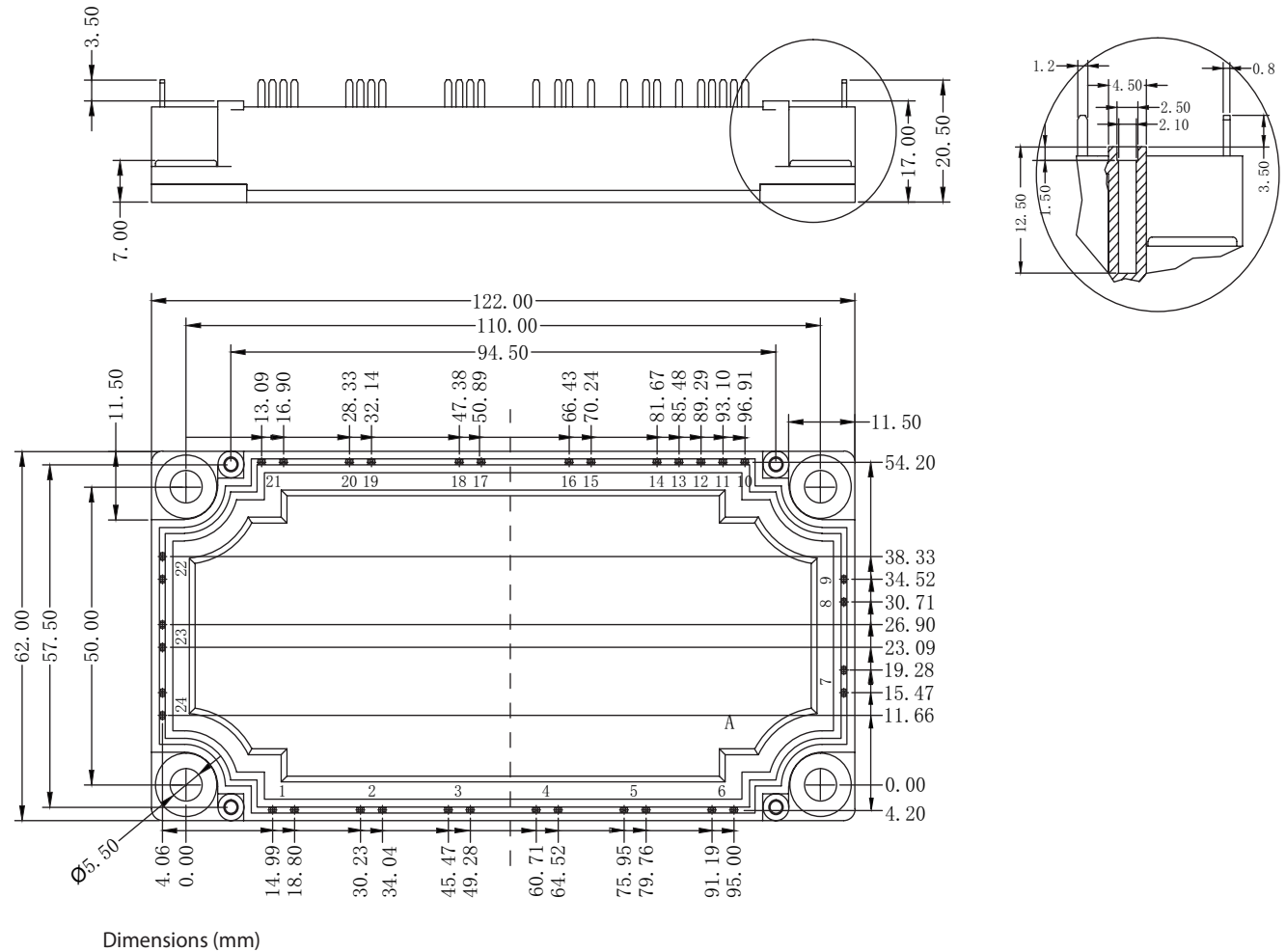
Dimensions (mm)
