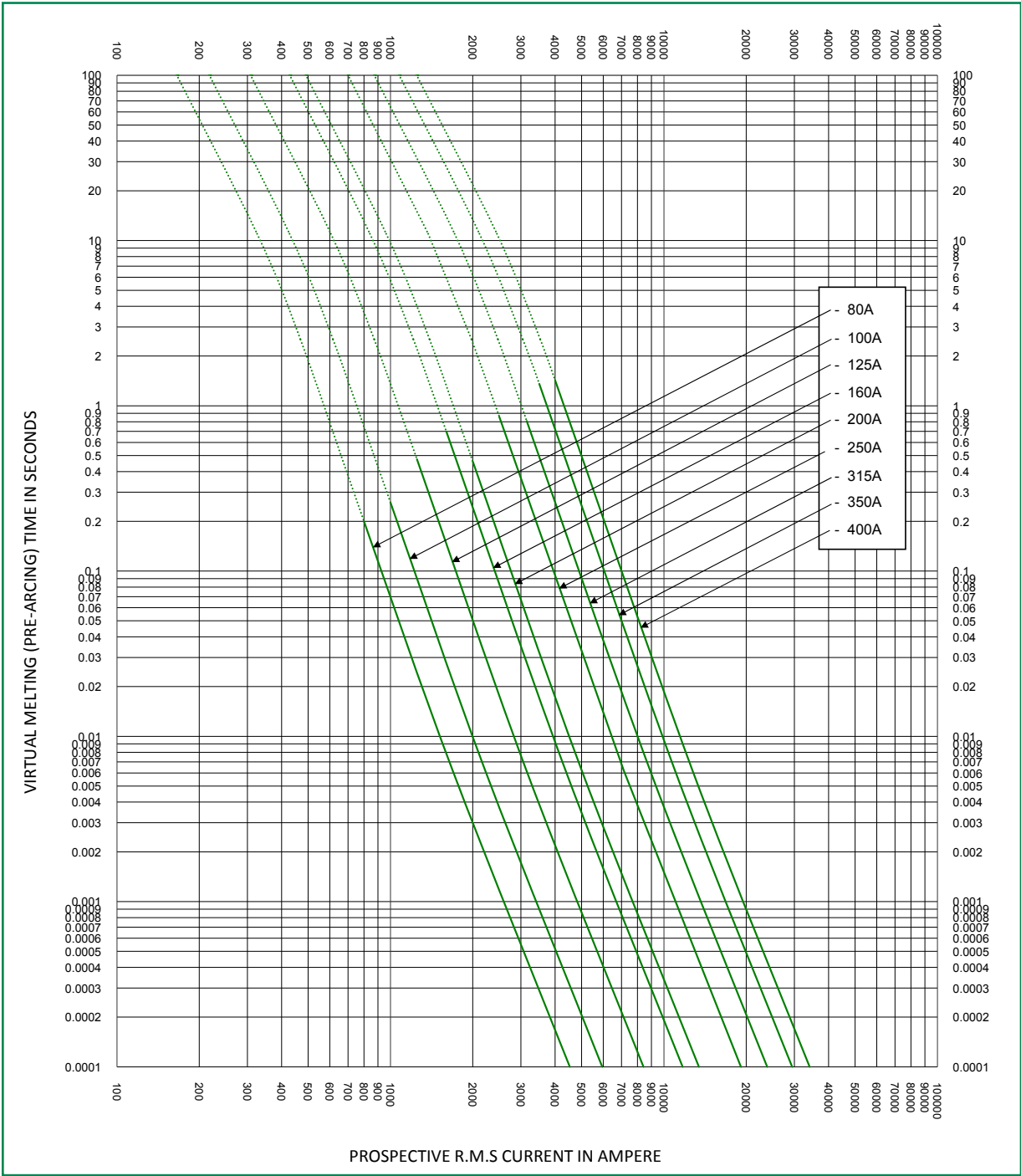
Time Current Curve (1XL Case Size 80 A–400 A)
