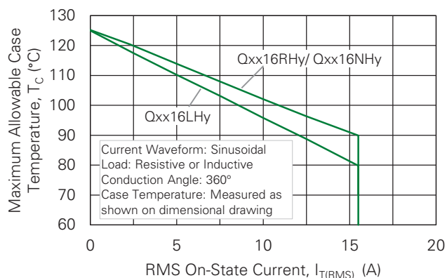
Fig. 7. Maximum Allowable Case Temperature vs. On-state Current (16 A Devices)
