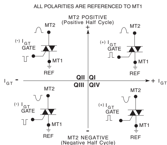
Figure 1. Definition of Quadrants
