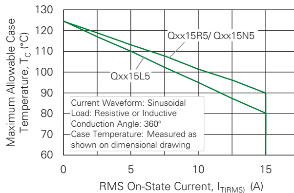
Fig. 6. Maximum Allowable Case Temperature vs. On-state Current (15 A Devices)
