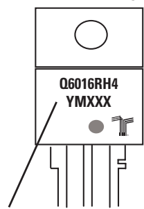
TO-220 AB - (L and R Package) TO-263 AB - (N Package)
