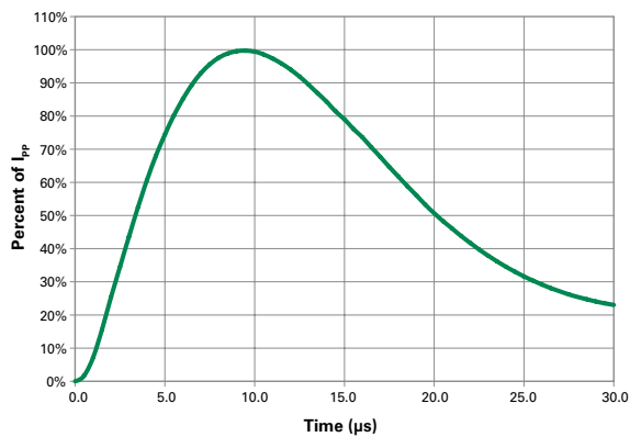
8/20 \mu s Pulse Waveform
